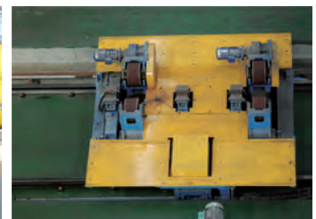
Turning Roll Machine
